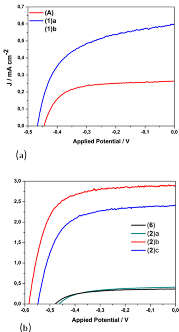
Fig. 13 J – V curves for the copper(I)-based dyes 1, [Cu(pqcame 2 )]PF 6 ] (A) (a); 2 and 6 (b). Lower case letters highlight the different architecture of the semiconductor material of the anode, dyed with 1 and 2, as reported in Table 2.
