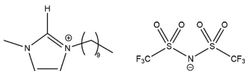
Fig. 5 Structure of ionic liquid [\text{C}_{10}\text{mim}][\text{NTf}_2] .
