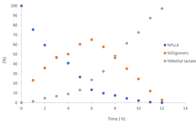
Fig. 5 Methanolysis of PLLA. Reaction conditions: 30 \mu mol of 4 , (0.6 mol% relative to ester linkages) in 10 mL of THF, with 1.2 mL of MeOH, T = 25 °C.
