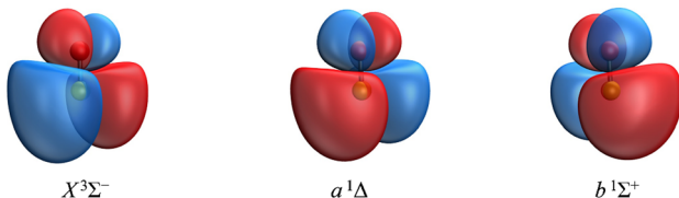
Fig. 3 The Dyson orbitals corresponding to detachment transitions from \text{SO}^- ( X^2\Pi ) to the X^3\Sigma^- , a^1\Delta , and b^1\Sigma^+ electronic states of neutral SO. The orbitals shown in (a) were calculated using transitions from EOM-EA-CCSD to EOM-SF-CCSD states, each starting from the common triplet-state reference, [\dots]^{22}(\pi\alpha)^1(\pi'\alpha')^1 , where \pi and \pi' are the canonical HOMOs of \text{SO}(X^3\Sigma^-) and [\dots]^{22} is the closed-shell configuration comprised of 22 electrons. The orbitals in (b) were obtained using EOM-IP-CCSD, starting from the [\dots]^{22}(\pi\alpha)^1(\pi\beta)^1(\pi'\alpha')^1 anion reference. The two orbitals for the a^1\Delta state shown in (a) describe the degenerate [\dots]^{22}(\pi\alpha)^1(\pi\beta)^1(\pi'\alpha')^1 \rightarrow [\dots]^{22}(\pi\alpha)^1(\pi\beta)^1 and [\dots]^{22}(\pi\alpha)^1(\pi'\alpha')^1(\pi'\beta')^1 \rightarrow [\dots]^{22}(\pi'\alpha')^1(\pi'\beta')^1 transitions accessible from the triplet reference. Only the former is accessible from the anion reference and hence only one a^1\Delta orbital is shown in (b). The calculations were done using the aug-cc-pVTZ+5s5p5d5f basis set at the CCSD(T)/aug-cc-pVTZ optimized geometry of the anion. Isosurface values 0.02.
