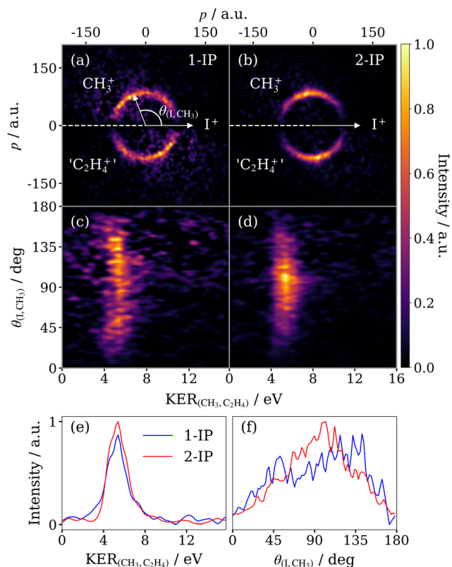
Fig. 7 Newton diagrams for the sequential breakup of (a) 1-IP^{3+} and (b) 2-IP^{3+} into ( I^+ + CH_3^+ + C_2H_4^+ ) in the COM frame of the secondary dissociation C_3H_7^{2+} \rightarrow CH_3^+ + C_2H_4^+ . The Newton diagrams are displayed in polar coordinates in (c) and (d) respectively, where KER_{(CH_3, C_2H_4)} is the KER of the secondary products and \theta_{(I, CH_3)} is the angle between the momenta of the iodine and methyl ions. Each panel is normalised separately. Below are overlaid the integrated KER (e) and angular distributions (f) for both isomers, normalised to unit area.
