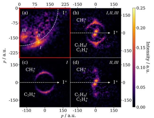
Fig. 6 (a) Momentum distribution of I^+ covariant with CH_3^+ , produced from the three-body breakup of 2-IP^{2+/3+} . The red box around this panel is to highlight the different scale for the momentum axes, and the different frame in which these data are presented. The three dissociation channels are as follows: (I) sequential three-body breakup of 2-IP^{3+} , (II) concerted three-body breakup of 2-IP^{3+} , (III) three-body breakup of 2-IP^{2+} . (b) Newton diagram for the same process, displaying the CH_3^+ momentum in the COM frame of the charged propyl intermediate. Filtering based on the absolute I^+ momentum has been used to isolate (c) the sequential breakup channel of 2-IP^{3+} ( 190 < p_{I^+} < 225 a.u.) from (d) the signal due to concerted breakup of 2-IP^{3+} as well as three-body breakup of 2-IP^{2+} ( 120 < p_{I^+} < 190 a.u.).
