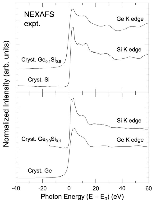
Fig. 2 Sensitivity of XAFS to backscattering environment. Top: Si K edge of crystalline Si and Ge K edge of a dilute Ge in Si crystalline \text{Ge}_{0.1}\text{Si}_{0.9} alloy. Bottom: Ge K edge of crystalline Ge and Si K edge of a dilute Si in Ge crystalline \text{Ge}_{0.9}\text{Si}_{0.1} alloy. The splitting of the white line (or “rabbit ears”) observed at the Si K edge is a density of states effect (see text). (After Woicik and Pianetta. 10 )
