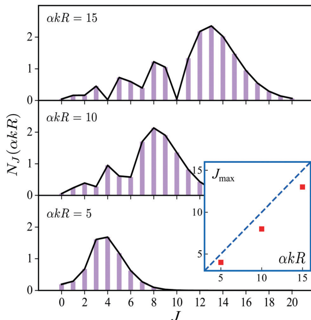
Fig. 2 Distribution N_J(\alpha_n R) (26) over J in the rotational recoil-induced wave packet (25) for different \alpha_n R . The red squares in the insert show the dependence of J_{\text{max}} on the recoil angular momentum \alpha_n R . Here J_{\text{max}} is the value of the angular momentum J when the distribution N_J(\alpha_n R) takes maximum. The dashed diagonal line in the insert corresponds to the recoil angular momentum J_{\text{rec}} = \alpha_n R (6).
