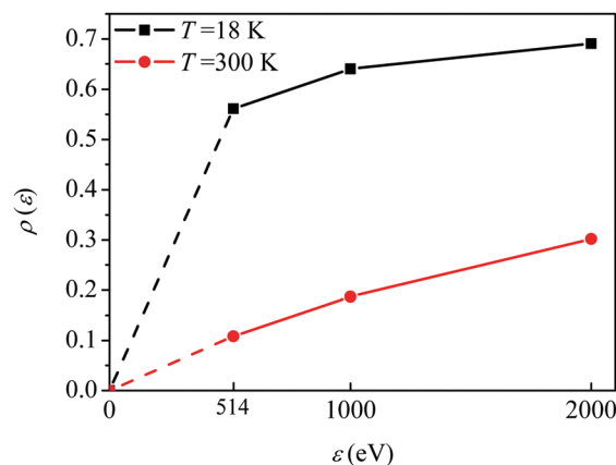
Fig. 10 The dependence of the visibility \rho(\varepsilon) (32) of the recoil-induced revivals on the energy of photoelectron \varepsilon . \alpha_C = 0.571 , \theta = 0 . The reason for \rho(0) = 0 is that the recoil-induced population of the rotational levels and, hence, the interference between intermediate rotational levels are absent when the momentum of the photoelectron fulfilled k = \sqrt{2\varepsilon} = 0 . The dashed lines connecting points \varepsilon = 514 eV and \varepsilon = 0 eV indicate that in the region 0 < \varepsilon \lesssim 500 eV the neglected Cohen-Fano interference can be significant.
