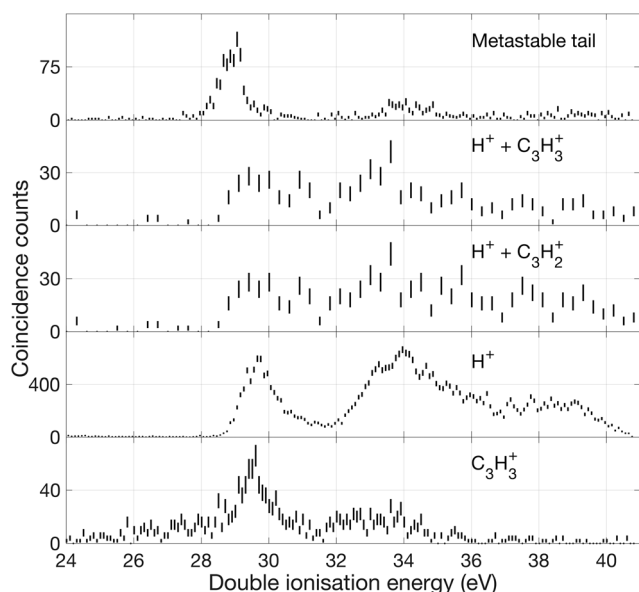
Fig. 12 Double ionization spectra based on electrons that were detected in coincidence with ions as specified in the figure. The uppermost spectrum represents decay events detected in the metastable tail shown in Fig. 7. The next lower spectra are derived from selection of events with two ions such as, \text{H}^+ and \text{C}_3\text{H}_3^+ , and two electrons, eei. The lower spectra are from events with one ion \text{H}^+ or \text{C}_3\text{H}_3^+ , respectively, and two electrons, eei. One coincident count is equivalent to two electrons being detected in the same event.
