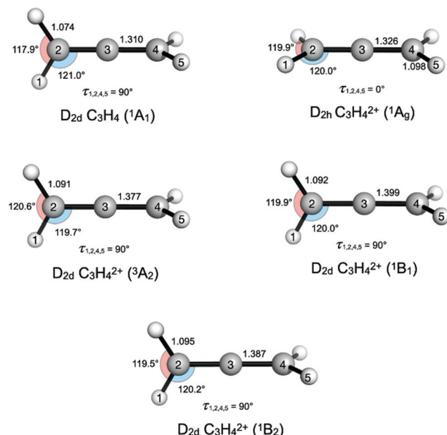
Fig. 1 Changes in electronic structure of neutral D_{2d} allene upon vertical double ionization (in eV) to the four lowest energy states to give: ^3A_2 , ^1A_1 , ^1B_1 and ^1B_2 that make up the first peak in the double ionization spectrum in Fig. 2. The D_{2d} ^1A_1 state undergoes a geometric distortion from D_{2d} \rightarrow D_{2h} to remove orbital degeneracy. Optimised geometries at the CASSCF/def2-TZVP level are shown, with distances in Å and angles in degrees.
