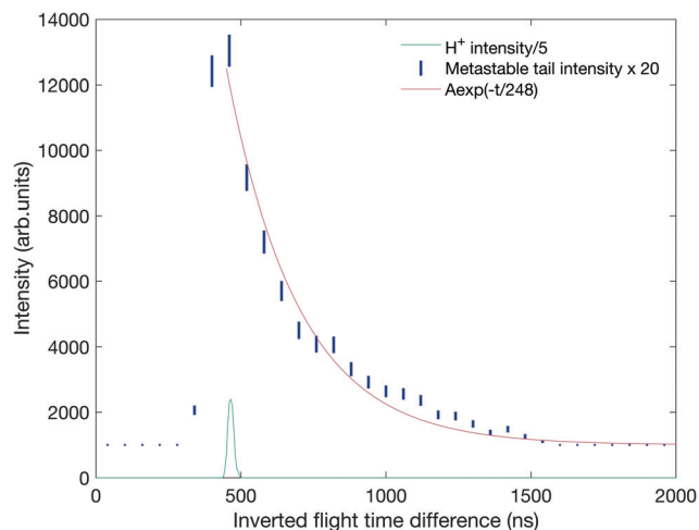
Fig. 8 Metastable tail intensity as a function of the inverted flight time difference with a fit to the exponential decay in red. The coincidences are the same as in the tail in Fig. 7 plotted against t_2 - t_1 where t_1 and t_2 are the flight times of the first and second ion to be detected, respectively. The location of the mass peak for \text{H}^+ ions on the same scale is included below the decay curve for comparison.
