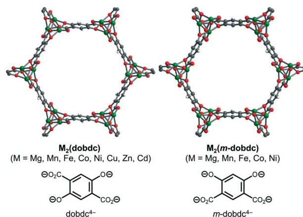
Fig. 1 Structures of M_2(\text{dobdc}) ( M = \text{Mg, Mn, Fe, Co, Ni, Cu, Zn} ; \text{dobdc}^{4-} = 2,5\text{-dioxidobenzene-1,4-dicarboxylate} , left) and M_2(m\text{-dobdc}) ( M = \text{Mg, Mn, Fe, Co, Ni} ; m\text{-dobdc}^{4-} = 4,6\text{-dioxido-1,3-dicarboxylate} , right). Green, gray, white, and red spheres correspond to magnesium, carbon, hydrogen, and oxygen, respectively.
