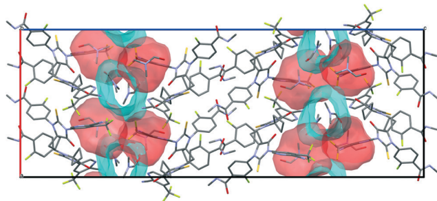
Fig. 10 Illustration of different types of voids coexisting in the crystal structures of APA-DMF-1:1.
