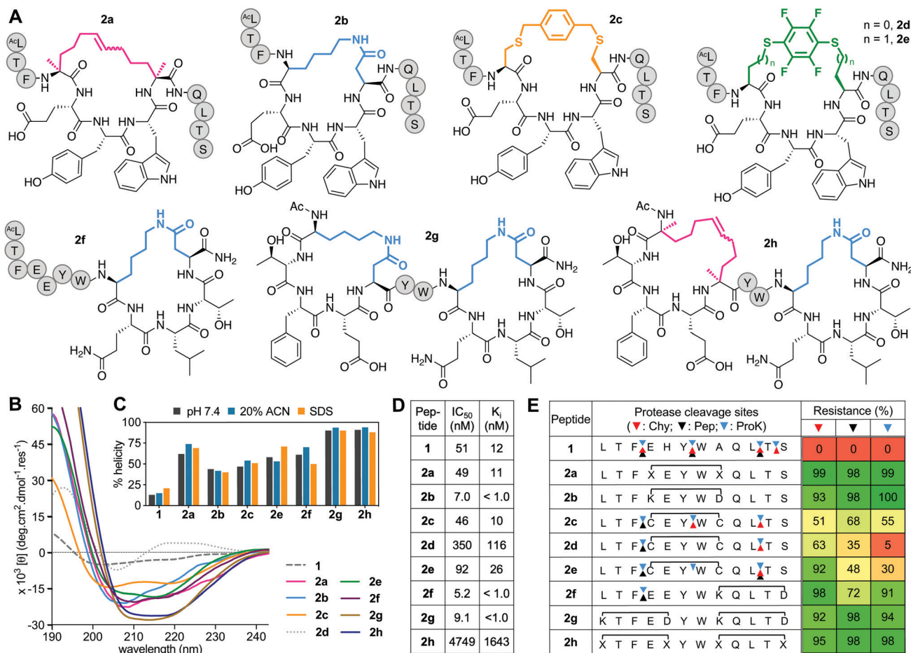
Fig. 2 A. Structures of (i \rightarrow i+4) -crosslinked peptides 2a – h . B. CD spectra for 2a – h vs. 1 (50 \mu M) in 10 mM phosphate buffer (pH 7.4) at 22 °C. C. Percent helicity calculated from CD spectra ( \theta_{220} ) in 10 mM phosphate buffer (pH 7.4), 20% ACN or 20 mM SDS buffer. D. IC_{50} = mean peptide concentration for inhibiting 50% binding of 1 -FITC (10 nM) to hDM2 (25 nM) measured by FP. pIC_{50} \pm SEM values are reported in Fig. S1 (ESI † ). Binding affinity ( K_i ) calculated from IC_{50} values. E. Heatmap indicating percent peptide intact after 2 h incubation with chymotrypsin (Chy), pepsin (Pep) or proteinase K (ProK) at 22 °C at pH 8 or 2 (Pep only), measured by LCMS. Arrows point to respective cleavage sites as revealed by LCMS analysis of the cleaved fragments.
