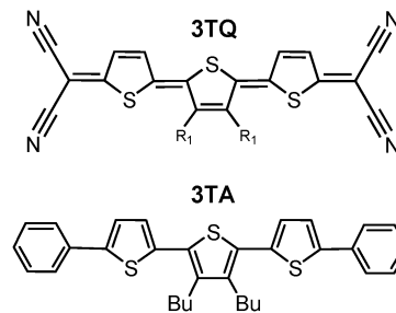
Scheme 4 Chemical structure of the quinoidal 3TQ in comparison with that of its aromatic counterpart, 3TA (Bu: n -butyl), a prototypical oligothiophene able to form \pi -dimeric dication.
