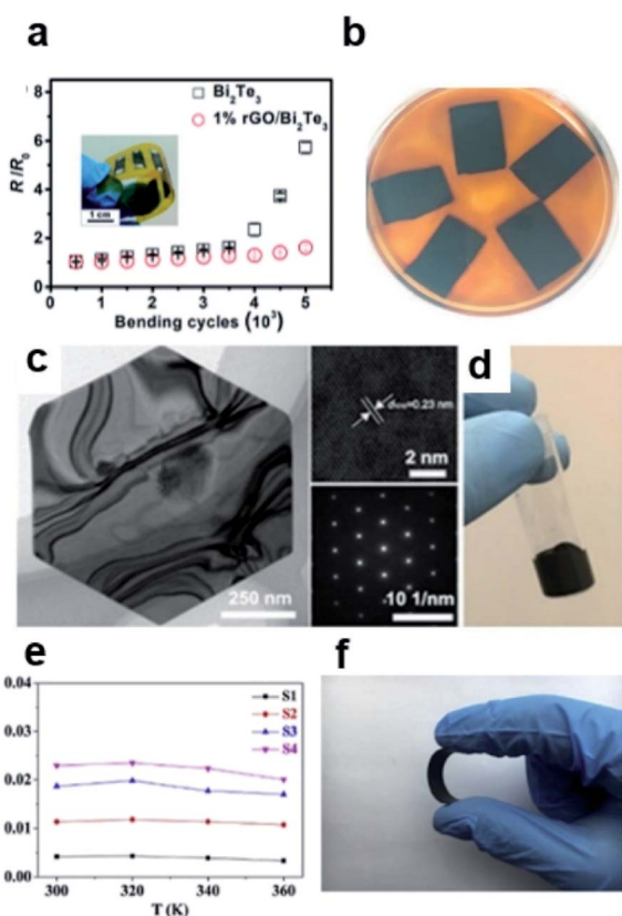
Fig. 6 (a) R/R_0 of a 1% rGO/Bi 2 Te 3 device with a bending radius of 5 mm ( R and R_0 are the resistances before and after bending, respectively). The R value of the 1% rGO/Bi 2 Te 3 device after 1000 bendings is 1/5 of the R value of the Bi 2 Te 3 device. rGO/Bi 2 Te 3 devices show excellent flexibility. Reproduced from ref. 64 with permission from the Royal Society of Chemistry. (b) GO film reduced by copper. Reproduced from ref. 65 with permission from Elsevier. (c) TEM and HRTEM of Bi 2 Te 2.7 Se 0.3 nanoplates. Reproduced from ref. 66 with permission from John Wiley and Sons. (d) Physical image of synthetic ink. (e) The ZT values of different CB/BTBA/PLA samples vary with temperature. (f) Flexibility of CB/BTBA/PLA composite materials. Reproduced from ref. 69 with permission from Elsevier.
