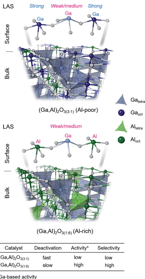
Fig. 5 Schematic representation of the distribution of bulk metal sites ( M_{IV} and M_{VI} , M = \text{Ga, Al} ) in (\text{Ga,Al})_2\text{O}_{3(3:1)} and (\text{Ga,Al})_2\text{O}_{3(1:6)} catalysts as well as the representative surface sites in these materials. The nature of surface metal sites and their Lewis acidity is linked to their performances in PDH.
