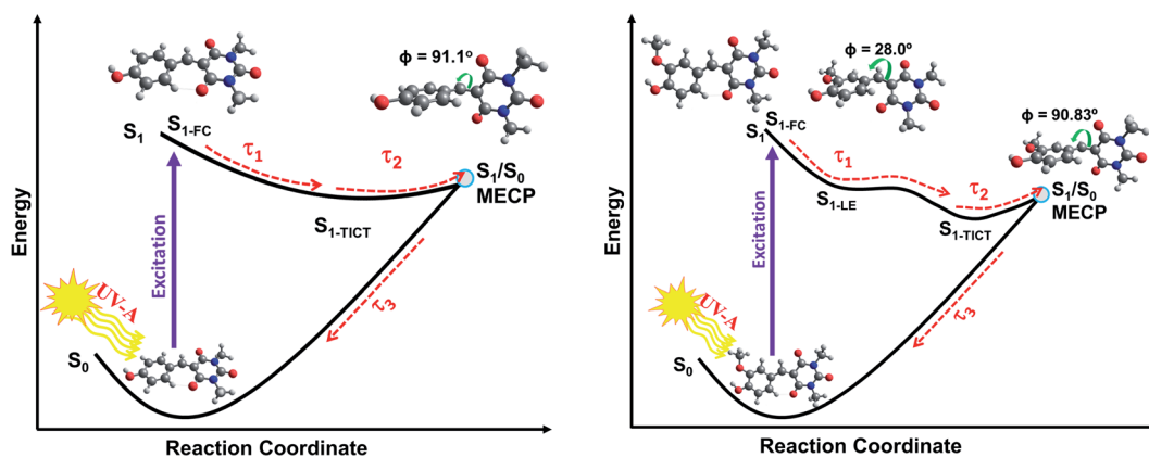
Fig. 5 Schematic of the relaxation pathways for CDBA (left) and FDDB- anti (right) representing the coumaryl and ferulyl series, respectively. Molecular conformations at the Franck–Condon (FC) region, at the local S_{1-LE} minimum (only for FDDB- anti ) and at S_1/S_0 MECP are shown. The respective \phi (C1–C2–C3–C4) dihedral angles, (see Scheme 1 for atom numbering), are also indicated. The molecular structures for the S_{1-TICT} configurations are omitted here for clarity but are shown in ESI Fig. S43 and S44† and are very similar to the respective S_1/S_0 MECP geometries.
