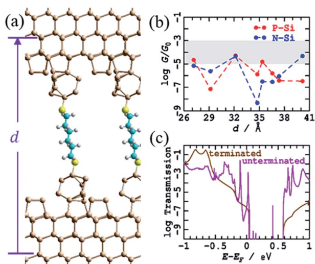
Fig. 4 Modelling the STMBJ experiment, using regular unterminated silicon tips on each unterminated electrode. (a) 2D ( 3 \times 3 ) model for tips spanned by Si(CH 2 ) 6 S at d = 37.37 Å; Si–brown, S–yellow, C–cyan, H–white. (b) Conductivity at zero voltage for P-type and N-type silicon at 0 K; the shaded region shows the observed conductance found throughout extensions of 3–10 Å for P-type Si. See ESI† Fig. S4 for more information. (c) Comparison of the transmission for P-type Si, as a function of electron energy from the Fermi energy, at d = 32.17 Å, from this unterminated series to that for the analogous terminated structure (Fig. 3, ESI† Fig. S3).
