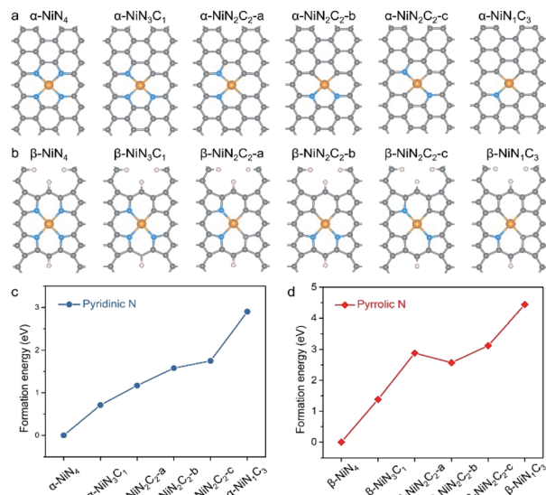
Fig. 1 Twelve different N-coordinated single-atom Ni configurations: (a) the commonly studied pyridinic-type Ni moieties in literature, \alpha\text{-NiNi}_x\text{C}_{4-x} ( x = 1-4 ); (b) the pyrrolic-type Ni moieties, \beta\text{-NiNi}_x\text{C}_{4-x} . The grey, blue, orange, and white spheres represent C, N, Ni, H atoms, respectively. Calculated formation energy of (c) \alpha\text{-NiNi}_x\text{C}_{4-x} and (d) \beta\text{-NiNi}_x\text{C}_{4-x} . The formation energy values of \alpha\text{-NiNi}_4 and \beta\text{-NiNi}_4 are set as zero.
