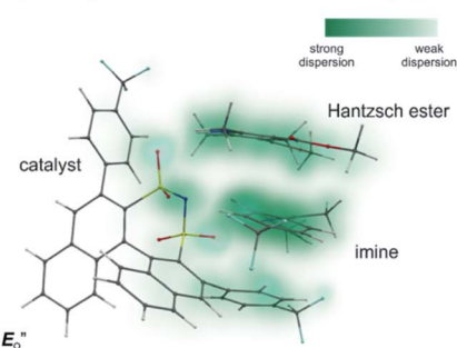
Fig. 4 (A) E_O'' and E_{N,I} shown here are the computed lowest-energy conformations of the ternary complex \text{CF}_3\text{-DSI } 2b/E\text{-}5b/3c . E_O'' accommodates all the experimental NOE and HOESY connections (key NOEs/HOEs are shown in the structures computed at TPSS-D3(BJ)/def2-SVP/SMD). Table 1 shows \Delta G_{(\text{DCM},180\text{ K})} for the principal conformations (free energy corrections and solvation corrections at the geometry optimization level of theory were added to the single-point total electronic energies). Table 2 illustrates the relative stabilities \Delta G_{(\text{DCM},180\text{ K})} of the conformationally refined structures. (B) Binding of the Hantzsch ester occurs at the oxygen atoms as evidenced by electrostatic potential map of the binary E_N and ternary E_O complexes. (C) Noncovalent interaction plot of complex E_O'' , suggesting that dispersion contributes significantly to stabilization of the ternary complex. (D) Dispersion interaction density plot confirms the importance of dispersion within complex E_O'' (computed at DLPNO-CCSD(T)/def2-TZVP level of theory).
