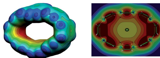
Fig. 13 3D (left) and 2D cross-section (right) of the MEP for the n\text{OK}[\text{8}]\text{CPP}^{4-} model (PBE0/cc-pVTZ).
