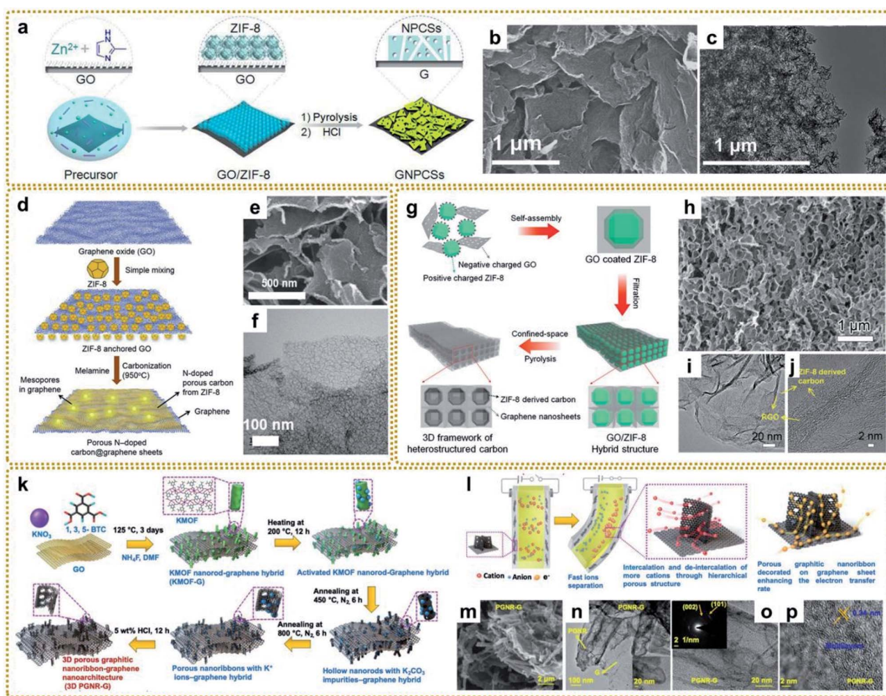
Fig. 5 (a) Illustration of the fabrication procedure for GNPCCs. (b) SEM and (c) TEM images of GNPCCs-800. Reproduced with permission from ref. 113. Copyright 2014, Wiley-VCH. (d) Graphical representation of the synthesis procedure of mesoporous-rich nitrogen-doped carbon anchored graphene sheets (MPNC@G) using melamine. (e) SEM and (f) TEM images of MPNC@G-1. Reproduced with permission from ref. 123. Copyright 2019, Elsevier. (g) A schematic illustrating the preparation of a PCF. (h) SEM, (i) TEM, and (j) HRTEM images of a PCF. Reproduced with permission from ref. 121. Copyright 2019, Wiley-VCH. (k) Schematic illustration of the synthesis of a 3D porous graphitic nanoribbon–graphene hybrid (3D PGNR–G) under solvothermal conditions followed by controlled pyrolysis processes. (l) Schematic illustration of the actuation mechanism for remarkable bending actuators based on a 3D PGNR–G/PEDOT:PSS electrode owing to fast ion mobility as well as electron transport through the hierarchical porous structure of the designed 3D PGNR–G in PEDOT:PSS. (m) FESEM image of 3D PGNR–G showing the anchoring of PGNR on wrinkled graphene sheets. (n) TEM image of 3D PGNR–G showing the decoration of PGNR on graphene sheets. The inset is an HRTEM image of 3D PGNR–G. (o) and (p) HRTEM images of 3D PGNR–G showing the presence of multilayered PGNR and graphene. The inset of (o) is its corresponding SAED pattern. Reproduced with permission from ref. 124. Copyright 2020, Wiley-VCH.
