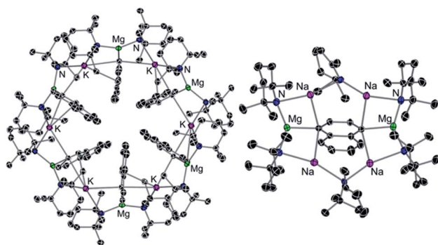
Fig. 2 Molecular structures of alkali-metal magnesiates \{[KMg(TMP)_2(C_{10}H_7)]_6\} ( 7 ) (LHS) and \{[Na_4Mg_2(TMP)_4(TMP^*)_2](1,4\text{-}C_{10}H_6)]\} ( 9 ) (RHS) resulting from AMMMg of naphthalene by [MMg(TMP)_2Bu] ( M = K , 6 ; M = Na , 8 ).
