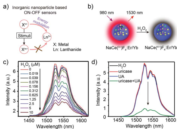
Fig. 4 Inorganic nanoparticles for biosensing in the NIR-II window. (a) Schematic illustration of inorganic nanoparticle-based sensing. (b) Schematic illustration of \text{NaCeF}_4\text{:Er}^{3+}/\text{Yb}^{3+} nanoparticles for \text{H}_2\text{O}_2 bio-sensing. (c) NIR-II luminescence emission response of the \text{NaCeF}_4\text{:Er}^{3+}/\text{Yb}^{3+} sensor with the addition of \text{H}_2\text{O}_2 . Ex: 980 nm. (d) NIR-II luminescence spectra of the \text{NaCeF}_4\text{:Er}^{3+}/\text{Yb}^{3+} sensor after the addition of \text{H}_2\text{O} , uricase, UA, and uricase + UA, respectively. Reproduced from ref. 56 with permission from the Royal Society of Chemistry, Copyright 2018.
