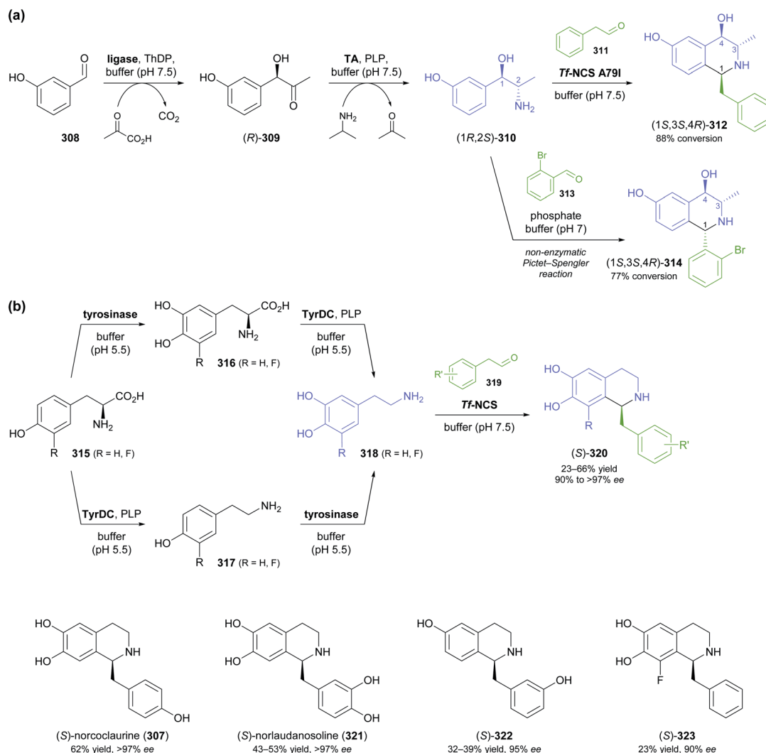
Scheme 40 In situ formation of amine substrates for norcoclaurine synthase: (a) combination of biocatalytic carboligation and transamination leads to metaminalol ( 310 ), which can undergo enzymatic or phosphate-catalysed Pictet–Spengler reactions. (b) Tyrosinase and tyrosine decarboxylase (TyrDC) can be used to prepare dopamine and its derivatives from the corresponding amino acids.
