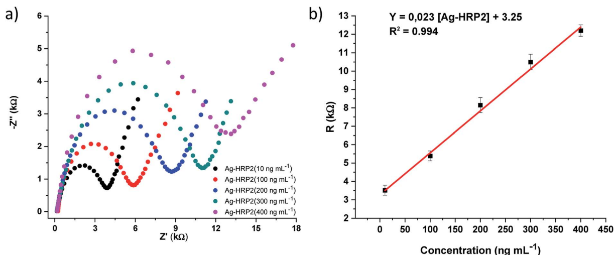
Fig. 5 (a) EIS spectra recorded with the Ab-PfHRP2/DHP/GE electrochemical immunosensor upon additions of Ag-PfHRP2 (10, 100, 200, 300, and 400 ng mL -1 ), (b) calibration curve: Y = 0.023 [Ag-PfHRP2] + 3.25 , with an R^2 = 0.994 .
