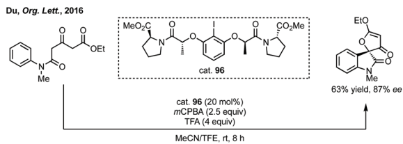
Scheme 64 Chiral hypervalent iodine mediated asymmetric spirocyclisation.
