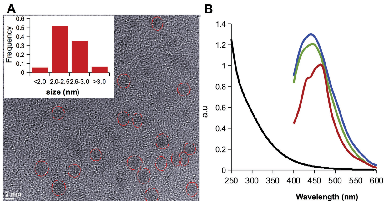
Fig. 3 (A) HRTEM image of LCND-2Na showing the size distribution (inset). (B) UV-Vis absorption (black line) and photoluminescence emission (excitation at 326 nm) spectra of LCD-1Na (green), LCD-2Na (blue) and CD-1Na (red).
