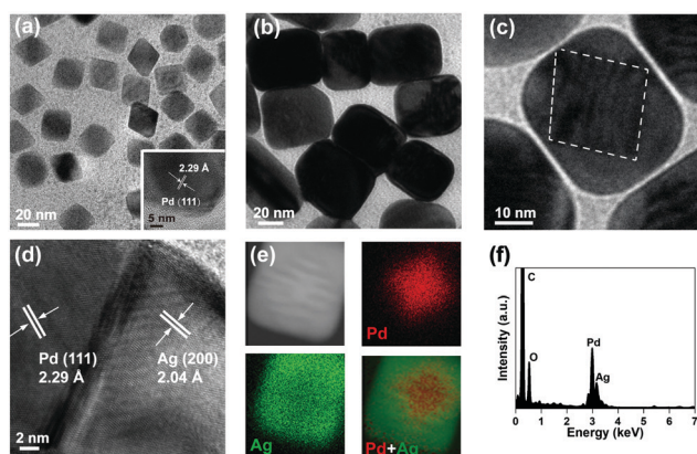
Fig. 1 Structural characterization of Pd Octs and Pd@Ag cubes. (a) TEM image of Pd Octs. (b and c) TEM and (d) HR-TEM images, (e) elemental mapping (raw data are displayed as Fig. S1, ESI†) and (f) the corresponding EDS profile of a Pd@Ag cube.
