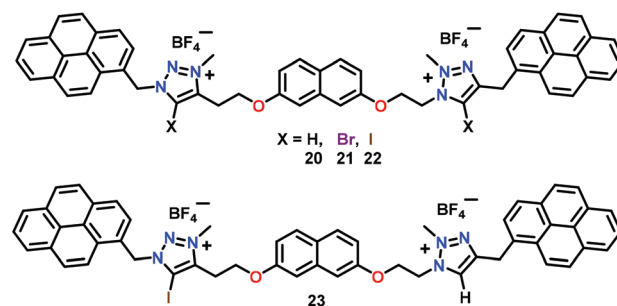
Fig. 10 Chemical drawings of chemosensors 20 – 23 . Adapted from ref. 54.
