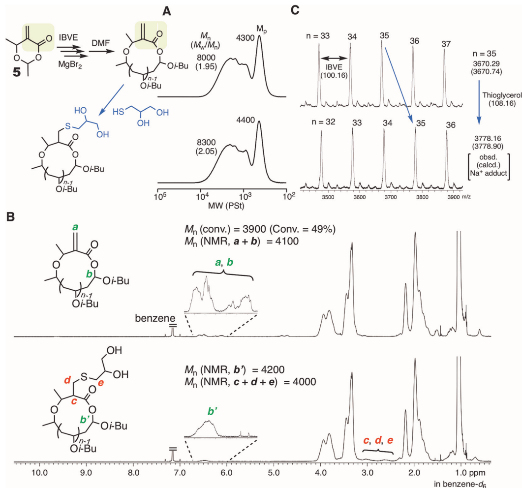
Fig. 6 Ring-expansion cationic polymerization of IBVE with 5 and \text{MgBr}_2 , and the post-polymerization reaction of the vinylidene group with thio-glycerol. (A) SEC; (B) ^1\text{H NMR} ; (C): MALDI-TOF-MS [\text{IBVE}]_0/[\mathbf{5}]_0/[\text{MgBr}_2]_0/[\text{DTBMP}]_0 = 380/5.0/5.0 or 10/0.15 mM in toluene/ \text{Et}_2\text{O} (90/10 vol%) at 0^\circ\text{C} . The sample was obtained at 49% conversion (1 hour). See the ESI† for the conditions of the post-polymerization reaction.
