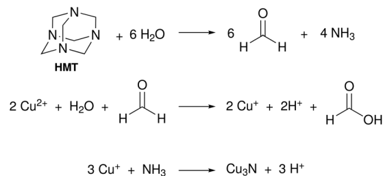
Fig. 17 Proposed reaction mechanism for \text{Cu}_3\text{N} formation from hexamethylenetetraamine and \text{Cu(NO}_3)_2 \cdot 5\text{H}_2\text{O} . 122
