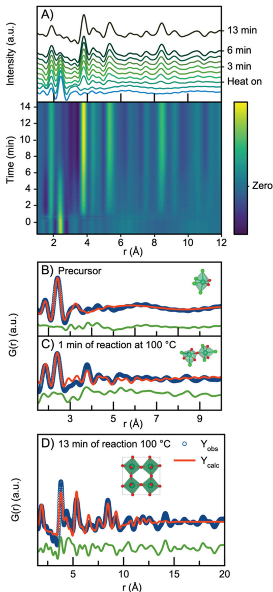
Fig. 8 (A) Time resolved PDFs collected at ambient pressure at temperature 100 °C. (B) Refinement of the precursor PDF using a single [NbCl 4 O 2 ] octahedra. (C) Refinement of the PDF collected at 1 min of reaction with a polyhedral cluster of [NbCl 6-x O x ] octahedra. (D) Refinement of PDF collected after 13 min of reaction using the ReO 3 structure.
