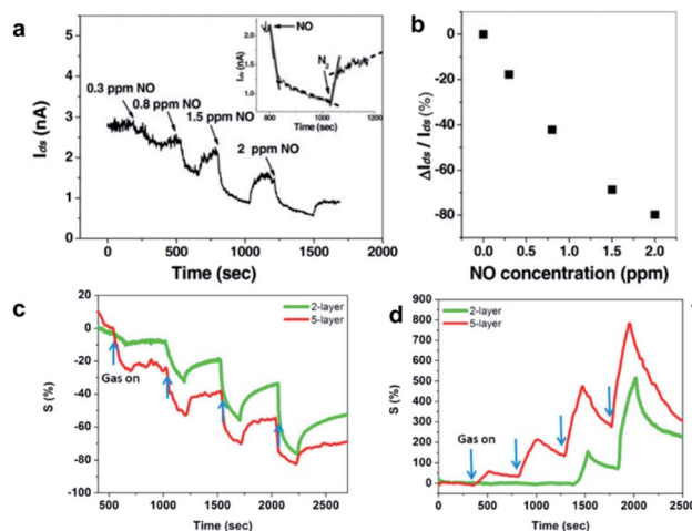
Fig. 11 (a) Real-time response upon exposure of the 2 L \text{MoS}_2 FET to \text{NO} with an increased concentration. Inset: typical adsorption and desorption process of \text{NO} molecules on the \text{MoS}_2 FET. (b) Plot of the percentage change of output current versus \text{NO} concentration. 83 Reproduced from ref. 83. Copyright 2012 John Wiley & Sons, Inc. Comparative 2 L and 5 L \text{MoS}_2 sensing performances in (c) \text{NH}_3 and (d) \text{NO}_2 of 100, 200, 500, and 1000 ppm, respectively. 84 Adapted with permission from ref. 84. Copyright 2013 American Chemical Society.
