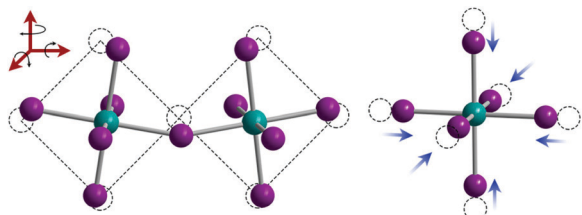
Fig. 10 Pressure-induced rotation of \text{PbI}_6 octahedra (left) and Pb–I bond compression (right). Reproduced with permission from ref. 160. Copyright 2017, American Chemical Society.
