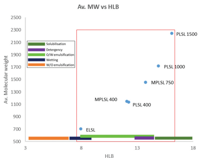
Fig. 7 HLB values and average molecular weight obtained for sophorolipid-based surfactants and their potential applications.
