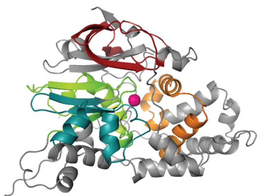
Fig. 1 Homology model of CtnHase. The four regions targeted by random mutagenesis are shown in colour. The cobalt ion is displayed as pink sphere, region \alpha 1 in blue, \alpha 2 in green, \beta 1 in orange and \beta 2 in red.
