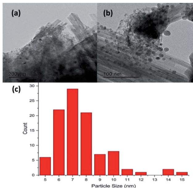
Fig. 2 Transmission electron micrographs of the as-received CuCl 2 /KCl/attapulgite catalyst: (a) scale bar = 200 nm, (b) scale bar = 100 nm. (c) TEM derived particle size distribution of the CuCl 2 particles.
