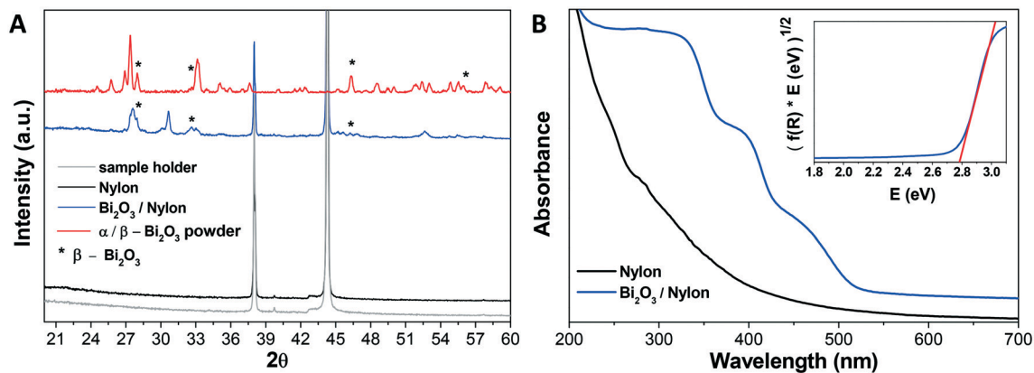
Fig. 2 A) XRD patterns of the sample holder, bare nylon, \text{Bi}_2\text{O}_3/\text{nylon} composite, and synthesized \alpha/\beta\text{-Bi}_2\text{O}_3 powder, and B) UV-vis DRS spectra of bare nylon and \text{Bi}_2\text{O}_3/\text{nylon} composite; inset: Tauc plot for the estimation of the bandgap.
