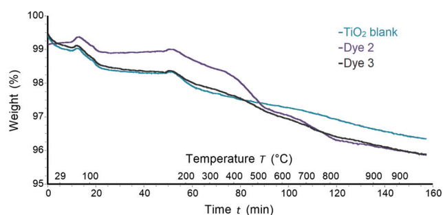
Fig. 7 TGA curves for blank TiO 2 (green), TiO 2 sensitized with dye 2 (purple) and TiO 2 sensitized with dye 3 (grey).
