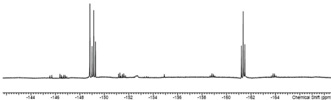
Fig. 6 The ^{19}\text{F}\{^1\text{H}\} NMR spectrum of [\text{SnF}_4(\text{dmsol})_2] (298 K) showing the resonances of the two isomers with ^{117/119}\text{Sn} satellites.
