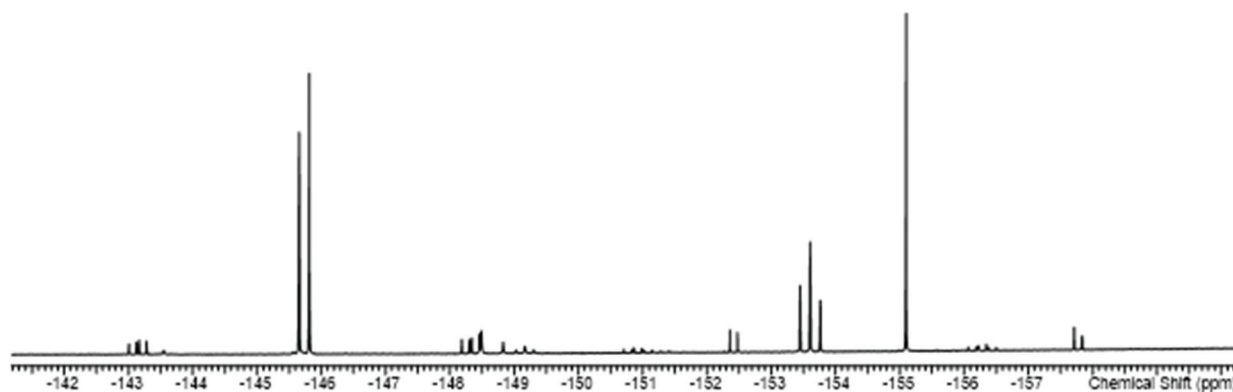
Fig. 7 The ^{19}\text{F}\{^1\text{H}\} NMR spectrum of [\text{SnF}_3(\text{dmsol})_3][\text{OTf}] (298 K) showing the resonances of the two isomers with ^{117/119}\text{Sn} satellites (the OTf resonance is not shown).
