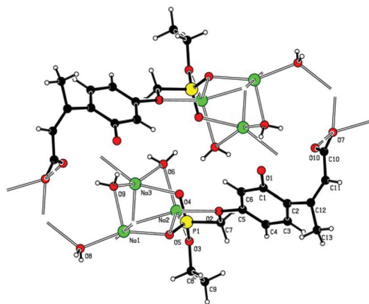
Fig. 5 X-ray structure of 2a trisodium 3-[4-(ethoxy-phosphonomethoxy)-2-phenolato]-but-2-enoate trihydrate. Left: showing \text{Na}^+ \cdots \text{O}-\text{P} , \text{Na}^+ \cdots \text{O}-\text{C} and \text{Na}^+ \cdots \text{OH}_2 bonding. Right: the extended hydrogen bonded chain structure.
