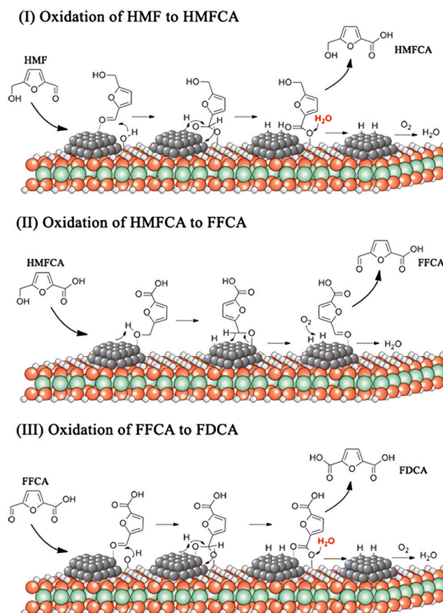
Fig. 7 View of the plausible reaction mechanism of oxidation of 5-HMF to FDCA over Pd/HT catalysts. Reprinted with permission from ref. 122, Copyright© 2016 American Chemical Society.
