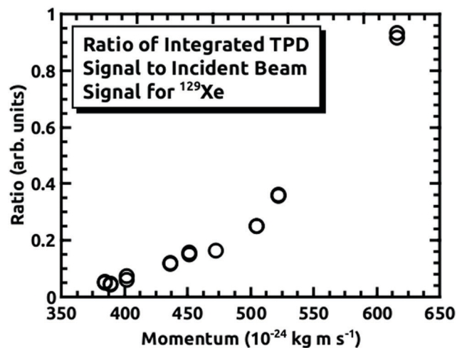
Fig. 3 Top panel: Thermal desorption spectra for the three Xe isotopes taken after a 45 minute exposure of the surface to D 2 O and Xe ( \langle v \rangle = 2.88 \times 10^3 m s -1 ) at \theta_1 = 10^\circ , with a linear ramp rate of 10 K min -1 . Lower panel: relative TPD intensities, normalized by the incident beam intensities, as a function of momentum for 129 Xe.
