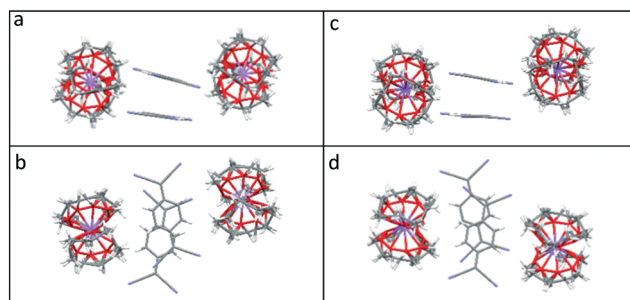
Fig. 2 Side (a) and top (b) views of the TCNQ 2- dimer in (12-crown-4) 2 LiTCNQ ( 1 ) in respect to the views (c and d) of (12-crown-4) 2 NaTCNQ ( 2 ).
