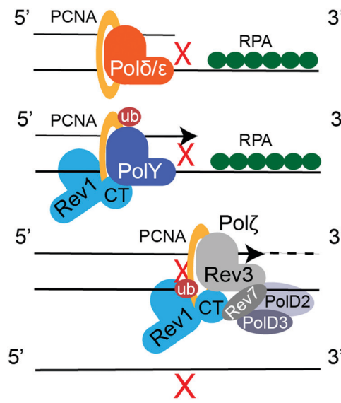
Fig. 8 Two step Rev1/Pol \zeta -dependent TLS. After PCNA monoubiquitination by Rad6/Rad18, an insertor Y-family TLS polymerase replaces a replicative polymerase, Pol \delta or Pol \epsilon , and inserts nucleotides across the DNA lesion. The extender TLS polymerase Pol \zeta continues replication past the site of DNA damage.
