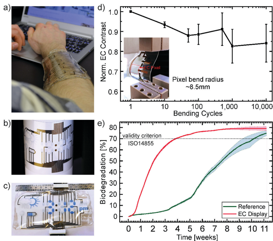
Fig. 4 (a) Photograph of the display attached directly onto the skin in an everyday-life situation demonstrating its wearability and transparency. (b) Photograph of the inkjet-printed displays highlighting the scalability and control of the process to produce a multisegment display. (c) The final display under operation showing the time, the battery status and sunny weather. (d) Electrochromic contrast (average of 3 devices) normalized to the starting value after bending the device several times by a bend radius of 8.5 mm. The inset shows a photograph of the bended device. (e) Biodegradation of the EC display and microcellulose (particle size 20 \mu\text{m} ) as a reference.
