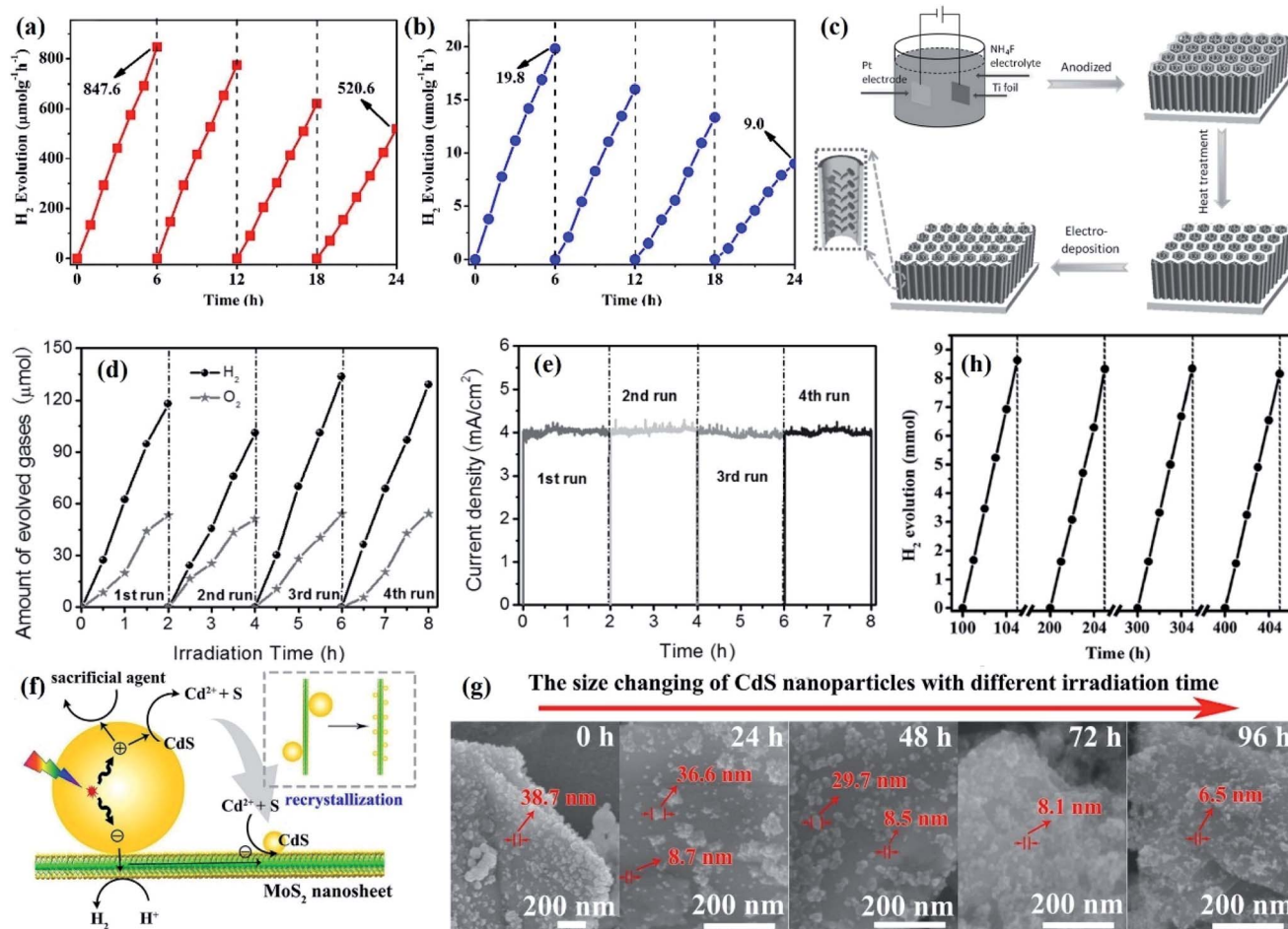
Fig. 8 (a) Stability test of CC-20 and (b) pristine CdS. The amount of hydrogen produced on CC-20 dropped to 520.6 μmol after 4 cycles of cycling tests, while that of pristine CdS dropped to 9.0 μmol. Reprinted with permission from ref. 130. Copyright 2018, Elsevier B.V. (c) Schematic illustration of the preparation of the hierarchical TiO 2 @CoNi-LDHs NTAs via an anodization and subsequent electrodeposition process for highly efficient and long-term stable PEC water splitting; (d) H 2 and O 2 evolution curves from the hierarchical TiO 2 @CoNi-LDH NTA electrodes at 1.23 V versus RHE under AM 1.5G for different cycles. (e) The steady-state photocurrent curve of the typical hierarchical TiO 2 @CoNi-LDH NTA electrode under AM 1.5G illumination at 1.23 V versus RHE for different cycles. Reprinted with permission from ref. 131. Copyright 2016, Wiley-VCH. (f) Schematic theories and the corresponding verification for the photocorrosion-recrystallization strategy of CdS in the 0D/2D CdS/MoS 2 nanocomposite; (g) morphology change of the CdS/MoS 2 nanocomposite at different visible light irradiation times; (h) H 2 evolution during the photocatalytic stability study for over 400 h. Reprinted with permission from ref. 139. Copyright 2016, Elsevier B.V.
