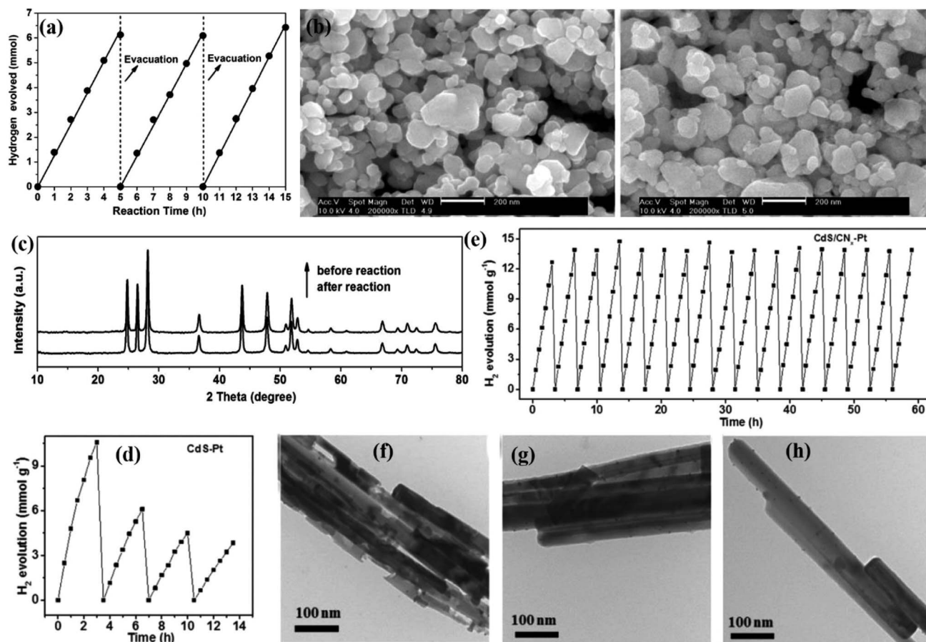
Fig. 2 (a) Time course of H 2 evolution on 0.9 mol% MoS 2 /CdS photocatalyst under visible light irradiation; (b) SEM images of 0.9 mol% MoS 2 /CdS prepared at 673 K and collected 0.9 mol% MoS 2 /CdS prepared at 673 K and (c) their XRD patterns. Reprinted with permission from ref. 53. Copyright 2012, Elsevier B.V. The catalytic stability of various photocatalysts for hydrogen production: (d) CdS-Pt and (e) CdS/CN x -Pt, respectively. TEM images of (f) CdS/Pt, (g) CdS-Pt/CN x and (h) CdS/CN x -Pt after cycled H 2 production. Reprinted with permission from ref. 54. Copyright 2017, Royal Society of Chemistry.
