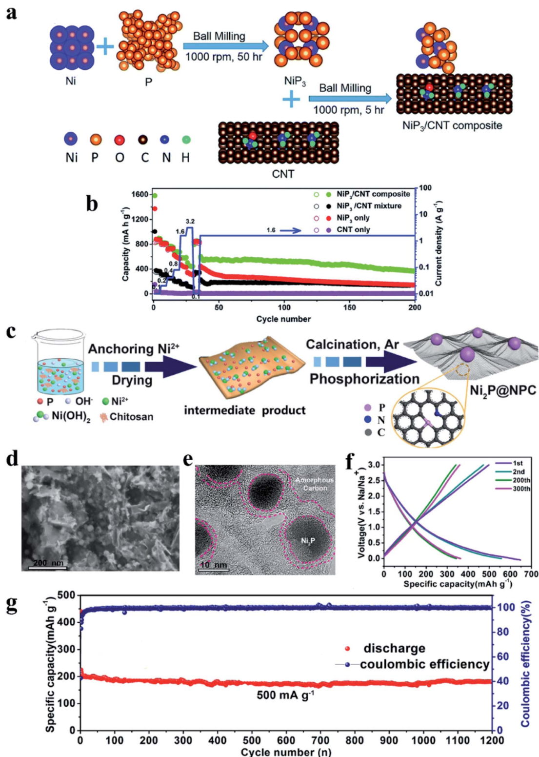
Fig. 24 (a) Schematic of the synthesis of the \text{NiP}_3/\text{CNT} composite. (b) Comparison of the cycling performances of \text{CNT} , \text{NiP}_3 , \text{NiP}_3/\text{CNT} mixture and \text{NiP}_3/\text{CNT} composite electrodes. Reproduced with permission. 226 Copyright 2018, The Royal Society of Chemistry. (c) Schematic of the synthesis of \text{Ni}_2\text{P}@NPC . (d) SEM and TEM images of \text{Ni}_2\text{P}@NPC . (e) HR-TEM image of \text{Ni}_2\text{P}@NPC . (f) Galvanostatic charge/discharge profiles of the \text{Ni}_2\text{P}@NPC SIB anode for the 1st, 2nd, 200th and 300th cycles respectively. (g) Long-term cycling stability and coulombic efficiency of the \text{Ni}_2\text{P}@NPC composite at 500 \text{ mA g}^{-1} . Reproduced with permission. 92 Copyright 2018, Elsevier Ltd.
