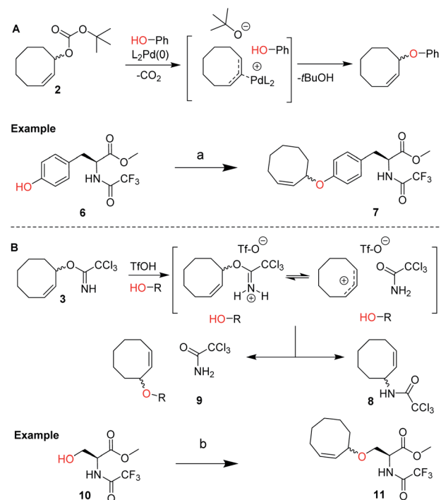
Scheme 2 (A) Design of cyclooctene tert -butyl carbonate reagent 2 for the palladium catalyzed installation of cyclooctene ethers on phenols, including the proposed mechanism based on the work of Grover and co-workers. 19 Reagents/conditions: (a) 2, Pd(PPh_3)_4 , dioxane, 80 °C, 80%; (B) design of cyclooctene trichloroimidate reagent 3 for the Lewis acid triggered formation of cyclooctene ethers from aliphatic alcohols. Proposed mechanism and products observed upon treating 3 with catalytic triflic acid are shown. Reagents/conditions: (b) 3, TfOH , DCM, -35 °C to 0 °C, 46% (Table S2†).
