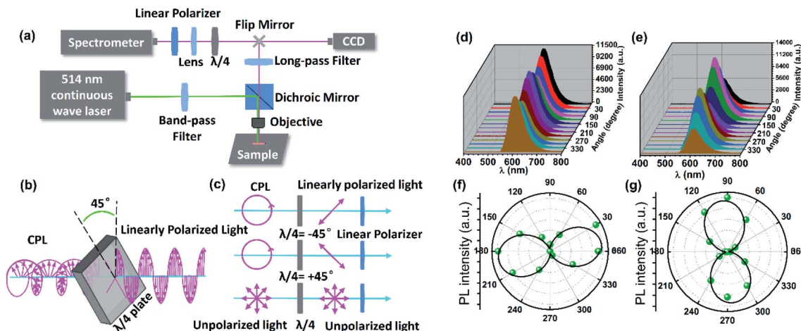
Fig. 3 (a) Schematic illustration of the experimental setup for measurements of micro-area CPL of single-crystal microrods of DSM@ P (+)-TbBTC. (b) Illustrative representation of the conversion between CPL and linearly polarized light through a \lambda/4 waveplate. (c) Evaluation of the circular polarization light. (d and e) Polarized emission spectra from one single-crystal microrod of DSM@ P (+)-TbBTC under 514 nm excitation at changed angles (0–360°), angles of the \lambda/4 waveplate = -45^\circ (d) and +45^\circ (e). (f and g) Maximum emission intensity of the same DSM@ P (+)-TbBTC microrod at different polarizer rotation angles, angles of the \lambda/4 waveplate = -45^\circ (f) and +45^\circ (g).
