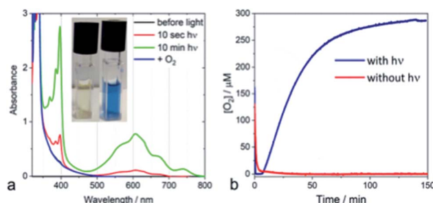
Fig. 2 (a) Spectral changes induced in an Ar-purged solution of nano-PDPB, 100 \mu\text{M} \text{MV}^{2+} , 10\% \text{TEOA} in MeCN by illumination with blue light and after aeration (inset: formation of the blue \text{MV}^{\bullet+} radical). (b) Time courses of oxygen evolution from water measured by a Clark electrode. Blue curve: with nano-PDPB (synthesized in mesophases) and red curve: no irradiation.
